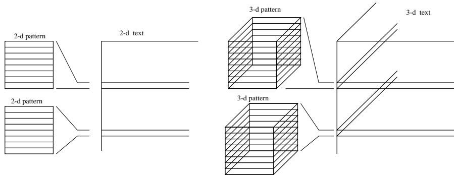
Figure 2: Algorithm for exact searching. All the pattern “rows” are searched in n/m text “rows” at the same time.
