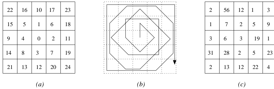
Figure 2: A spiral reading order for the sistring that starts in the middle of a text of size 5 \times 5 . Figure (a) shows the reading order by enumerating the cells, and figure (b) shows the enumeration graphically. Figure (c) shows the color values of the cells of the image, so for that image the sistring corresponding to the reading order is \langle 3, 2, 19, 2, 6, 7, 5, 5, 28, 3, 12, 1, 12, 13, 31, 1, 56, 1, 9, 23, 22, 2, 2, 3, 4 \rangle .
