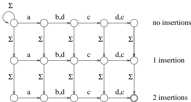
Figure 2. An NFA to search the superimposition "abcd" and "adcc" allowing 2 insertions.
