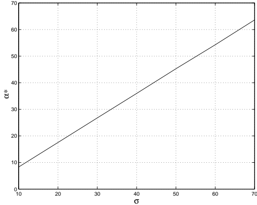
Figure 10. The \alpha^* limit as \sigma grows, for m = 300 .
