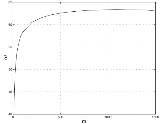
Figure 9. The \alpha^* limit as m grows.
