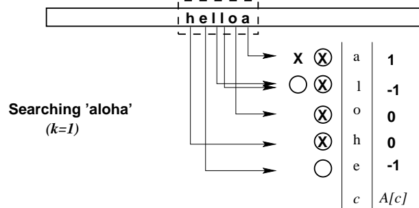
Figure 4. An example of the counting filter. The crosses represent elements which A[] accepts, and the circles are the elements that appeared in the window. A[c] stores crosses minus circles, and count counts circled crosses.
