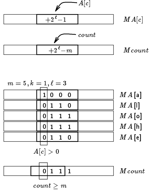
Figure 6. Scheme and an example of the bit-parallel counters. The example follows that of Figure 4.
