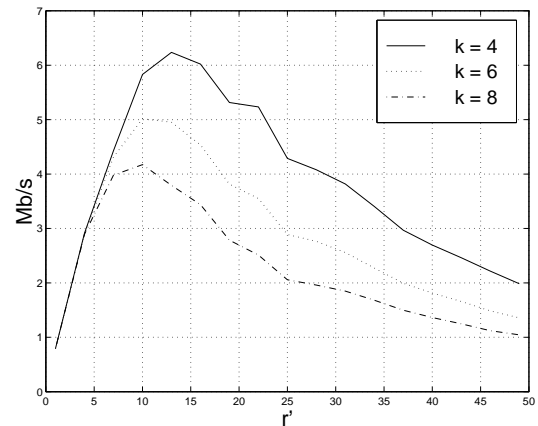
Figure 12. Mb/s vs partition size for k = 4 , k = 6 and k = 8 over a set of 100 patterns with m \in \{4, 5, 6\} .
