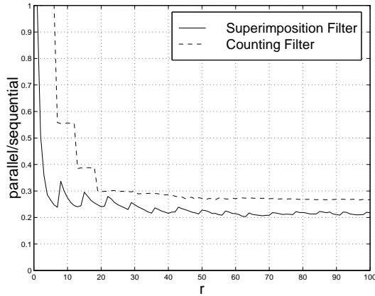
Figure 13. Ratio between parallel and sequential versions of the algorithms.
