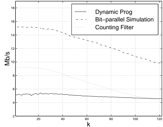
Figure 11. Scanning efficiency of the bit-parallel simulation and the counting filter compared to the classical dynamic programming algorithm.
