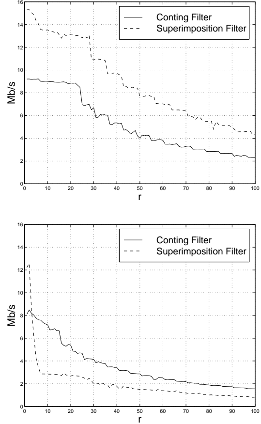
Figure 14. Mb/s processed by both algorithms for a set of patterns with m \in \{4, 5, 6\} with k = 4 (top) and k = 25 (bottom).
