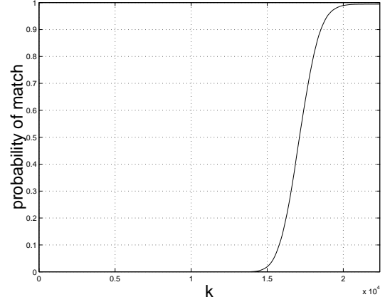
Figure 8. Matching probability for increasing k values and fixed m = 300 .
