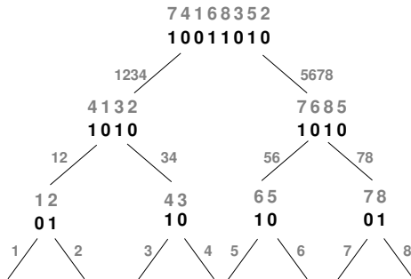
Figure 7: Representing permutation \pi = (7\ 4\ 1\ 6\ 8\ 3\ 5\ 2) using a wavelet tree. As before, the grayed values are not actually stored.
