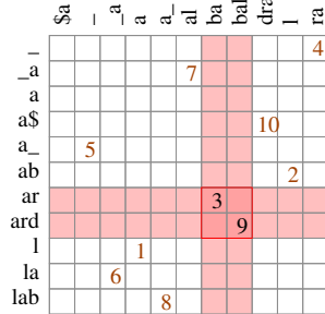
Figure 15: An LZ78 parsing of the text "alabar a la alabarda$", into 11 phrases. To find pattern "bar" split over phrases, we look for a phrase ending with "b" followed by another starting with "ar" (partition ("ba", "r") must also be tried). The grid connects those consecutive phrases: on the x coordinate, the reversed preceding phrases; on the y -coordinate, the following phrases. By sorting both sets in lexicographic order, the problem becomes a range search, where our pattern is found in phrases 3 and 9.
