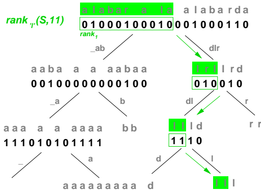
Figure 6: Computing \text{rank}_{l'}(S, 11) , that is, the number of occurrences of 'l' up to position 11 in S , using a wavelet tree, and finding out it is 2.
