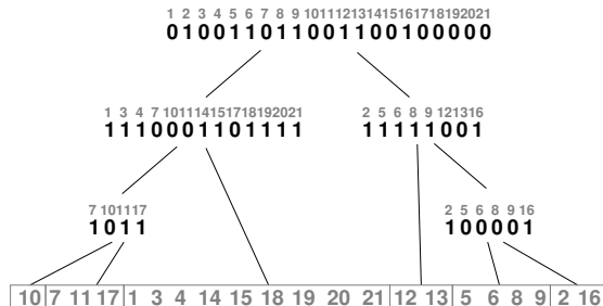
Figure 12: Representing a permutation with runs (on the bottom, the runs are shown with rectangles). Only the tree shape and the bitmaps, in black, are stored.
