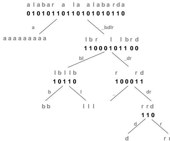
Figure 5: A wavelet tree with Huffman shape for our string S .
