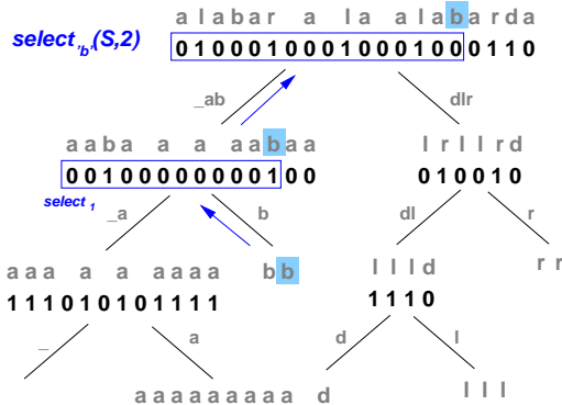
Figure 3: Tracking upwards to find the position of the second 'b' in S , finding it at S[16] . Recall that only the tree topology and the bitmaps are actually stored.
