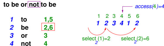
Figure 10: Representing text ‘to be or not to be’ with an inverted list (left) or with a wavelet tree (right). Words are mapped to 1, 2, 3, 4 and the wavelet tree represents the sequence of mapped words. Then we access any text word (e.g., the 4th text word is 4, or ‘not’), and successive \text{select}_2 operations retrieve the content of the inverted list of word 2, or ‘be’.
