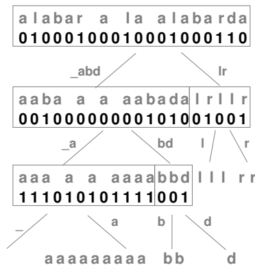
Figure 4: A pointerless wavelet tree. Now the tree topology (in gray, also surrounding the nodes in rectangles for clarity) is not represented; the structure just stores one bitmap per level and concatenates them. Note that the alphabet partition is slightly modified.
