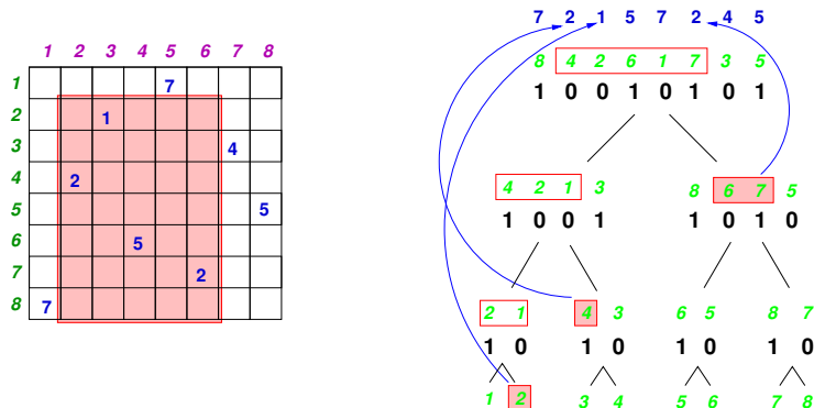
Figure 16: A grid with weights (left) and its wavelet tree representation (right). The wavelet tree represents the points; the weights are represented separately as an array on top, sorted by x -coordinate. A range is decomposed into maximal wavelet tree nodes (shaded), and the position of the minimum weight within each range is obtained. Then these positions are tracked to the top sequence to find the actual weights and give the global minimum, 1.
