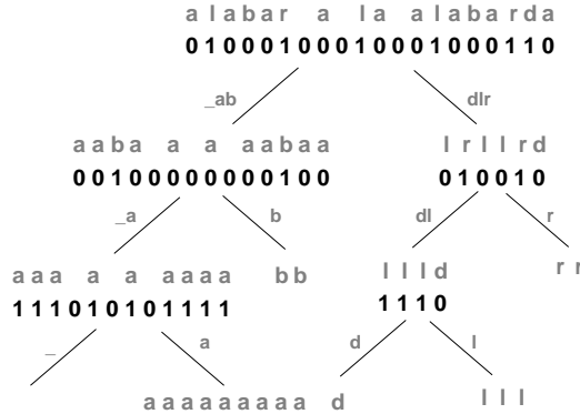
Figure 1: A wavelet tree on string S = \text{"alabar a la alabarda"} . We draw the spaces as underscores. The subsequences of S and the subsets of \Sigma labeling the edges are drawn (in gray) for illustration purposes; the tree stores only the topology and the bitmaps (in black).
