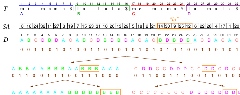
Figure 14: The suffix array SA of a collection, its document array D , and its wavelet tree representation on the bottom. A query for “ la ” yields an interval D[21, 25] , and the wavelet tree is used to spot all the different values of D in that interval.
