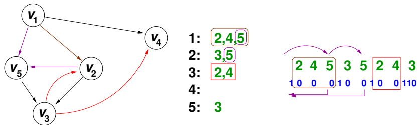
Figure 11: Representing a graph (left) with a wavelet tree plus a bitmap (right). The direct neighbors of v_3 are obtained by accessing part of the sequence (square-corner rectangle). The reverse neighbors of v_5 are found by successive select 5 operations (curved arrows, on top) and rank on the bitmap (straight arrows, on the bottom). The presence of an edge from v_1 to v_2 is decided via rank 2 in the area of the edges leaving v_1 (rounded-corner rectangle).
