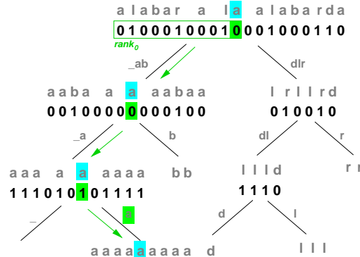
Figure 2: Accessing the symbol S[11] from our example wavelet tree, and finding out it is an 'a'. Recall that only the tree topology and the bitmaps are actually stored.
