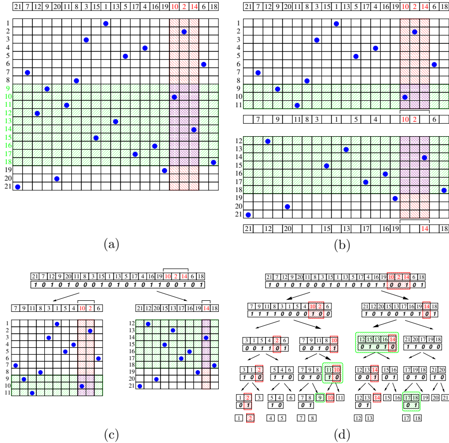
Figure 8: Representing a grid with a wavelet tree, and a range search. (a) The grid and the range as the intersection of an x - and a y -range. On top, the sequence of y -coordinates sorted by x -coordinate. The final structure is just the wavelet tree of that sequence. (b) Partitioning into small and large y -values, and the subsequences belonging to each partition. (c) First wavelet tree decomposition, at the root. The bitmap indicates to which partition each y -coordinate belongs, in x -coordinate order. (d) The final wavelet tree, indicating in bold arrows the edges traversed to count the points in the range. Nodes are followed as long as they contain some nonempty part of the x -range, they have nonempty intersection with the y -range, and are not contained in the y -range. We highlight the maximal nodes covering the query y -range (round-corner hatched boxes, in bold those reached), and the query x -range inside the sequence of each involved node (sharp-corner hatched boxes, in bold those traversed).
