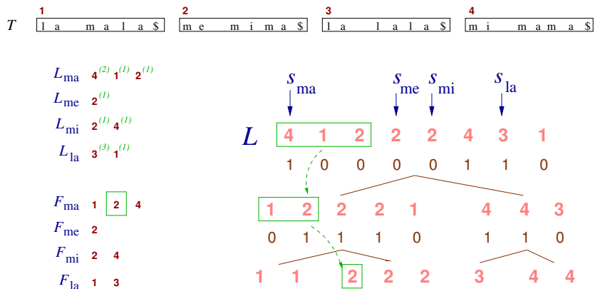
Figure 13: Representing a non-positional inverted list for a collection of four documents. The L lists are sorted by decreasing frequency; the F lists by increasing document identifier. The wavelet tree on the right represents both lists simultaneously. An L list is obtained by just accessing the sequence. An element of the F list (in this example, the 2nd element of the list F_{ma} ) by a range quantile query for the 2nd smallest value in the range. We first go left because there are 2 or more 0s in the range, then right because there are less than 2 0s.
