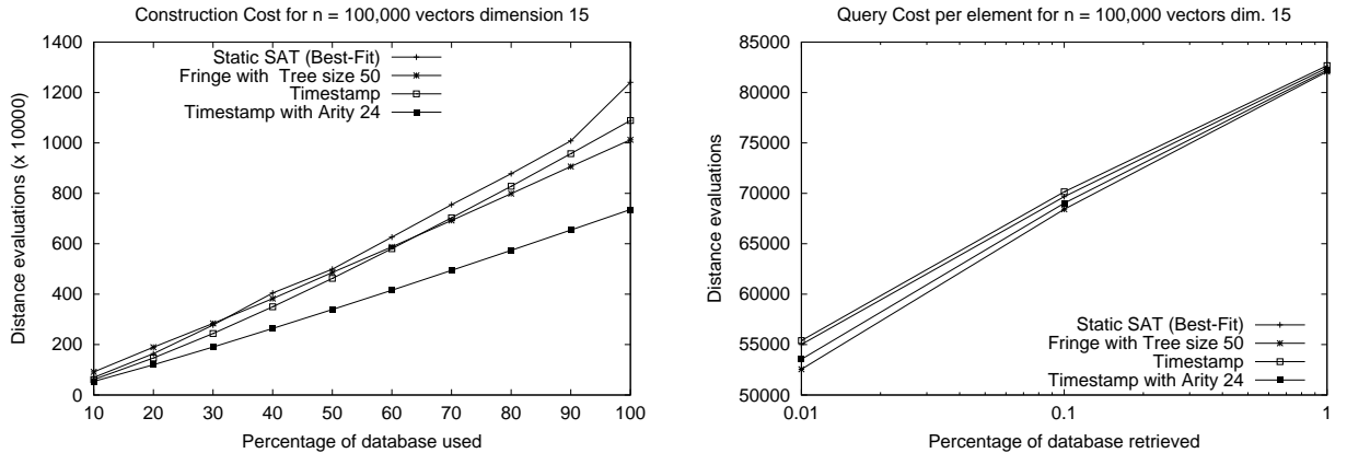
Figure 8: Construction and search costs for different methods in the sapce of vectors in dimension 15.
