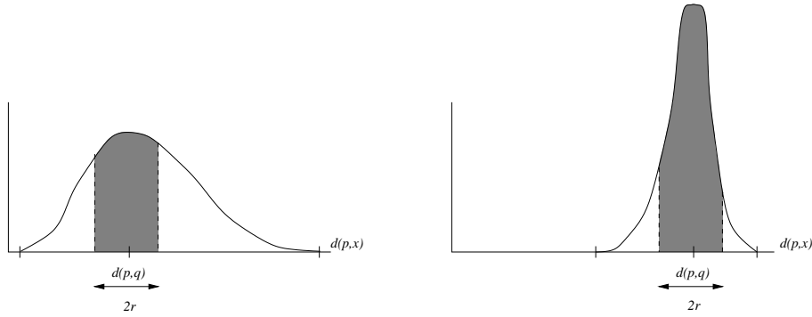
Fig. 14. A low-dimensional (left) and high-dimensional (right) histogram of distances, showing that on high dimensions virtually all the elements become candidates for the exhaustive evaluation. Moreover, we should use a larger r in the second plot in order to retrieve some elements.
