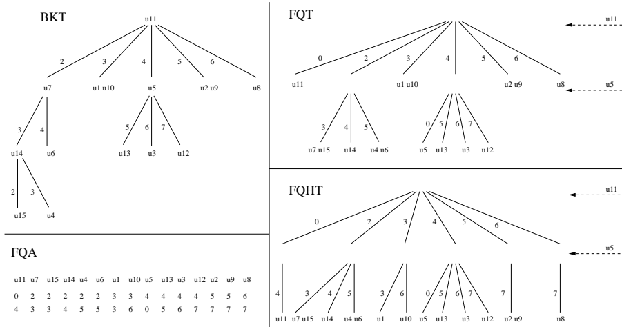
Fig. 3. Example BKT, FQT, FHQT and FQA for our set of points. We use b = 2 for the BKT and FQT, and h = 2 for FHQT and FQA.
