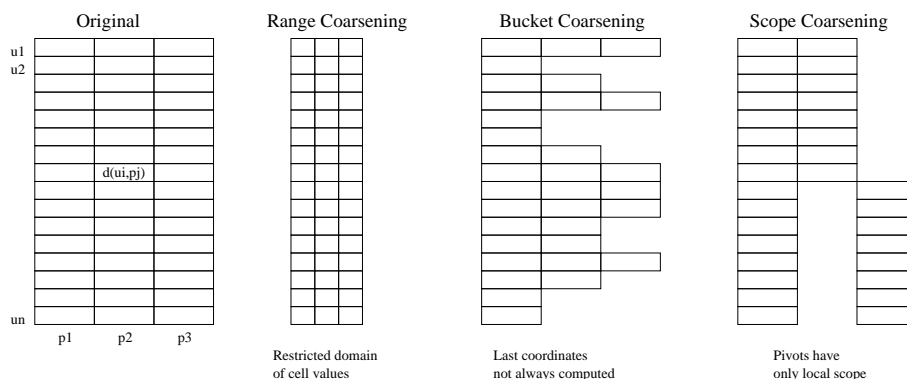
Fig. 21. Different coarsification methods.
