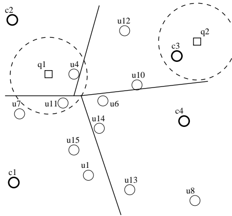
Fig. 13. A Voronoi partition using four centers and two query balls intersecting some classes. Note that the class of c_3 could be excluded from consideration for q_1 by using the covering radius criterion but not the hyperplane criterion, while the opposite happens to discard c_4 for q_2 .
