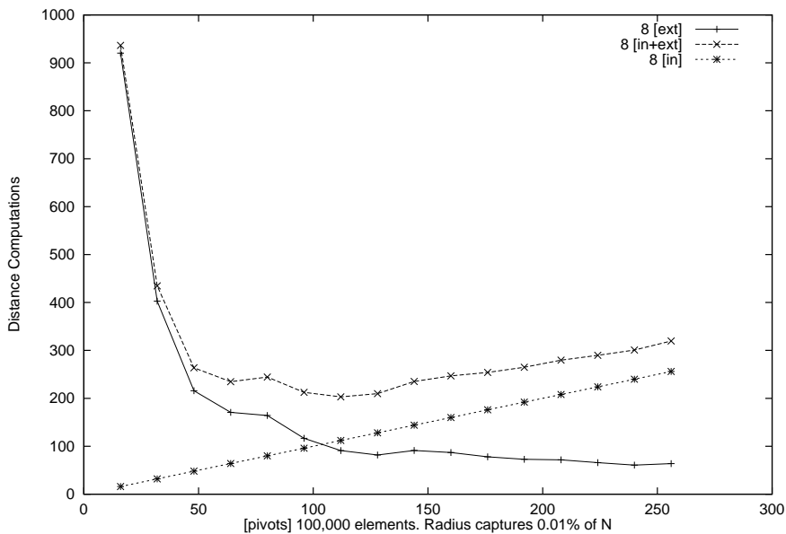
Fig. 15. Internal, external and overall distance evaluations in 8 dimensions, using different number of pivots k .
