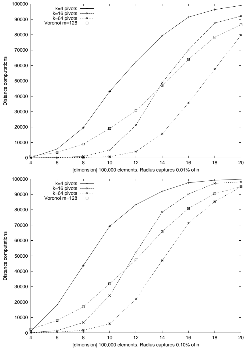
Fig. 19. Distance evaluations for increasing dimension. We compare the Voronoi algorithm of Figure 18 using 128 centers per level against the filtration using k pivots for k = 4, 16, 64 . On top the search radius captures 0.01% of the set, on the bottom 0.1%.
