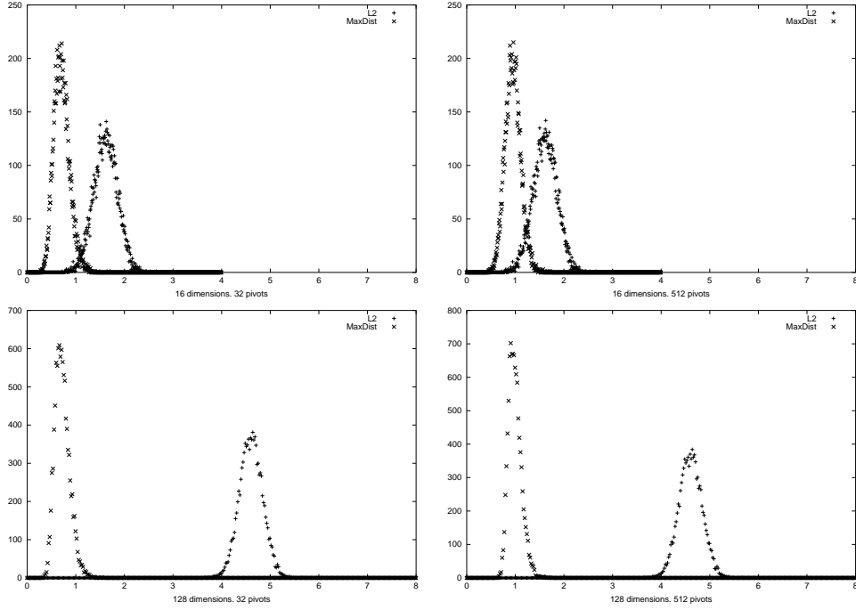
Fig. 17. Histograms comparing the L_2 distance in different \ell -dimensional Euclidean spaces and the pivot distance (MaxDist) obtained using different numbers k of pivots. In the top row \ell = 16 and in the bottom row \ell = 128 . On the left k = 32 and on the right k = 512 .
