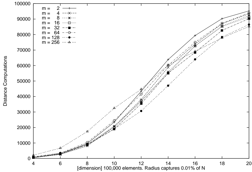
Fig. 18. Overall distance evaluations using a hierarchical Voronoi partitioning with different arities.
