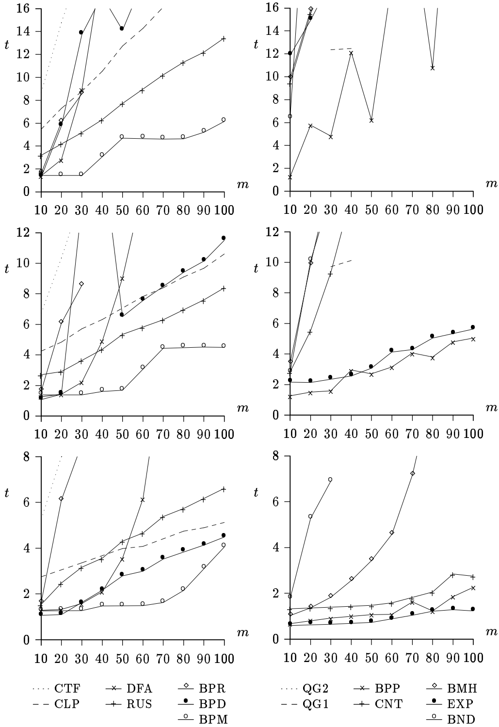
Figure 27: Results for \alpha = 0.3 and varying m . The left plots show non-filtering and the right plots show filtering algorithms. Rows 1 to 3 show DNA, English and speech files, respectively.
