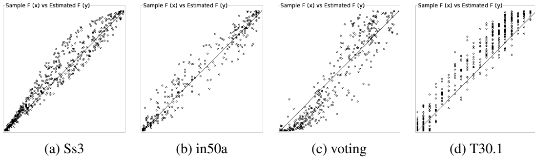
Figure 2: Scatter plots generated by Joint PDF Estimator.
