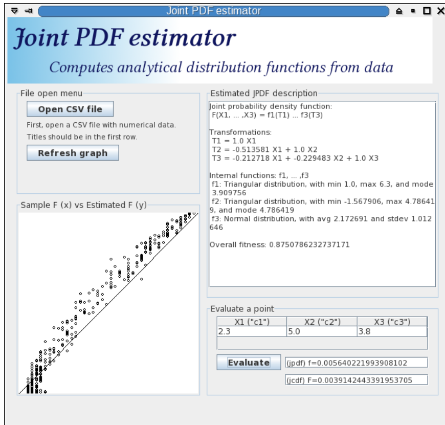
Figure 1: Joint PDF Estimator. Evaluated with cc42a dataset.
