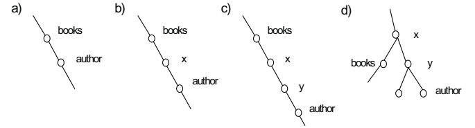
Figure 3: Sample fragments retrieved by BELOW (a), b), c) and NEAR (d) queries.
