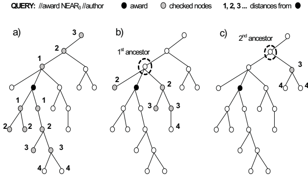
Figure 4: Example of NEAR constraint: a) BELOW operations, b) Descendants of 1 st ancestor, c) Descendants of 2 nd ancestor
