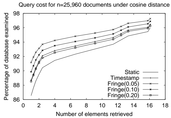
Figure 15: Comparison between the static and dynamic versions. At the top left, construction times in number of distance computations per element. The other plots refer to search times, in percentage of the database examined.
