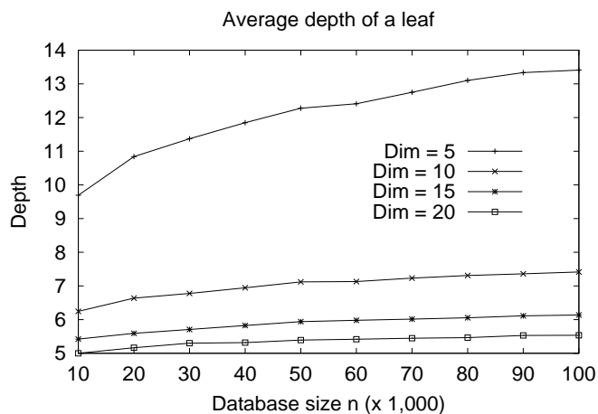
Figure 10: Average leaf depth in the tree. It grows with n and decreases with the dimension of the database. On the right, the formula obtained by least squares and the relative error.
