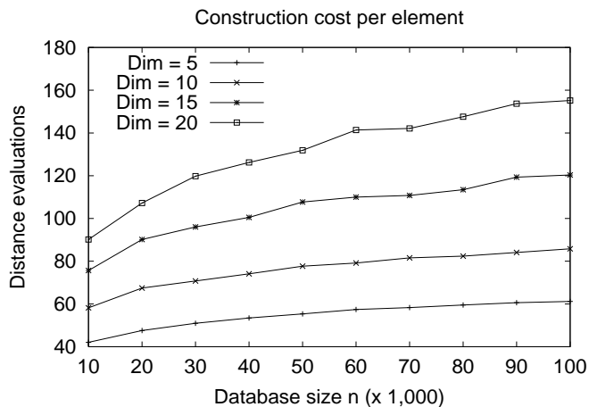
Figure 8: Construction cost, measured in number of distance evaluations per element. The cost grows with n and with the dimension of the database. On the right, the formula obtained by least squares and the relative error.
