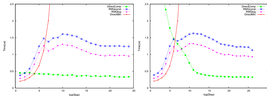
Figure 7: The files chr22.dna (left) and jdk13c (right). The behavior of DIRECTMIN , RMQ const , and RMQ log for the other other files in Manzini corpus (and pitches from Pizza&Chile ) is similar; the curve of DIRECTCOMP is in-between the two cases shown. The file jdk13c is the only one where the combination DIRECTCOMP-DIRECTMIN is slightly slower than RMQ log on a very small interval.
