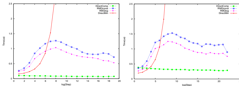
Figure 6: The files book1 (left) and E.coli (right). The behavior of DIRECTMIN , RMQ const , and RMQ log for the other three files from Canterbury corpus is similar; the curve of DIRECTCOMP (green) is in-between the two cases shown. (For files of size less than 1MB, DIRECTCOMP is the best on all inputs.)
