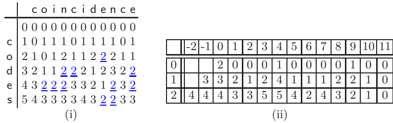
Figure 9: (i) Dynamic programming matrix for searching for the pattern codes in the text coincidence. The ends of the farthest reaching 2-paths are underlined. (ii) The rows containing the ends of the farthest reaching d -paths, 0 \leq d \leq 2 .
