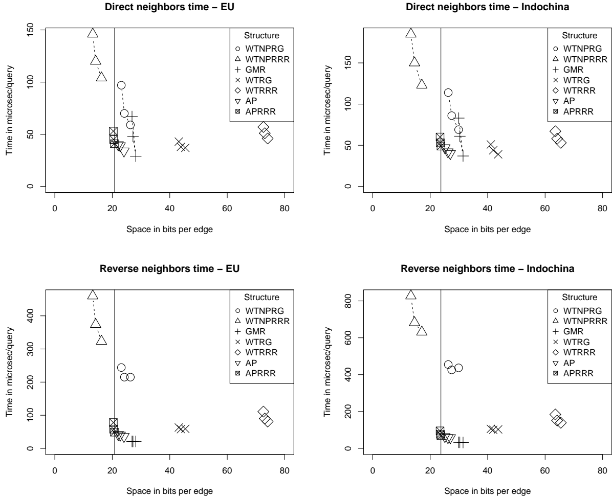
Figure 5: Performance on Web graphs, to retrieve direct and reverse neighbors. The vertical line marks the bits per edge required by a plain adjacency list representation.
