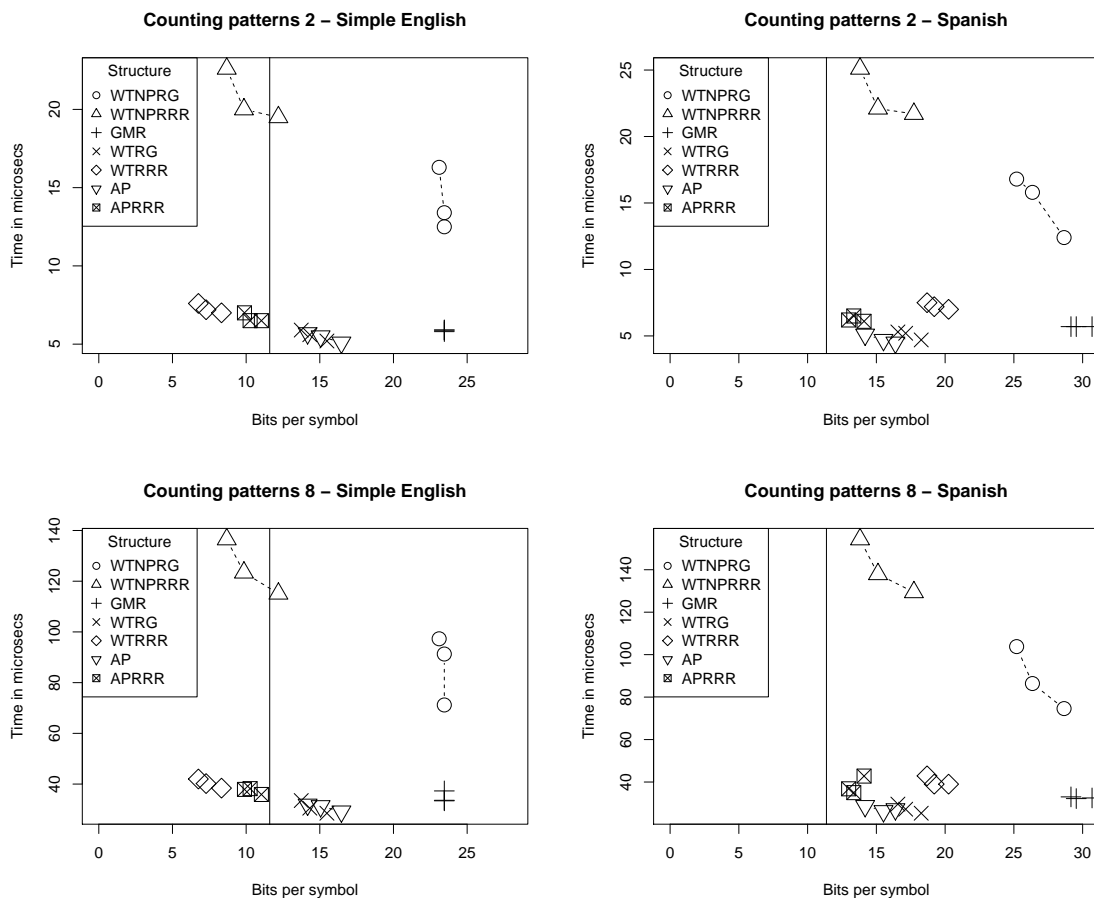
Figure 4: Time for counting queries on word-based FM-indexes. The vertical line marks the zero-order entropy of the sequences; remember that some schemes achieve high-order entropy spaces.
