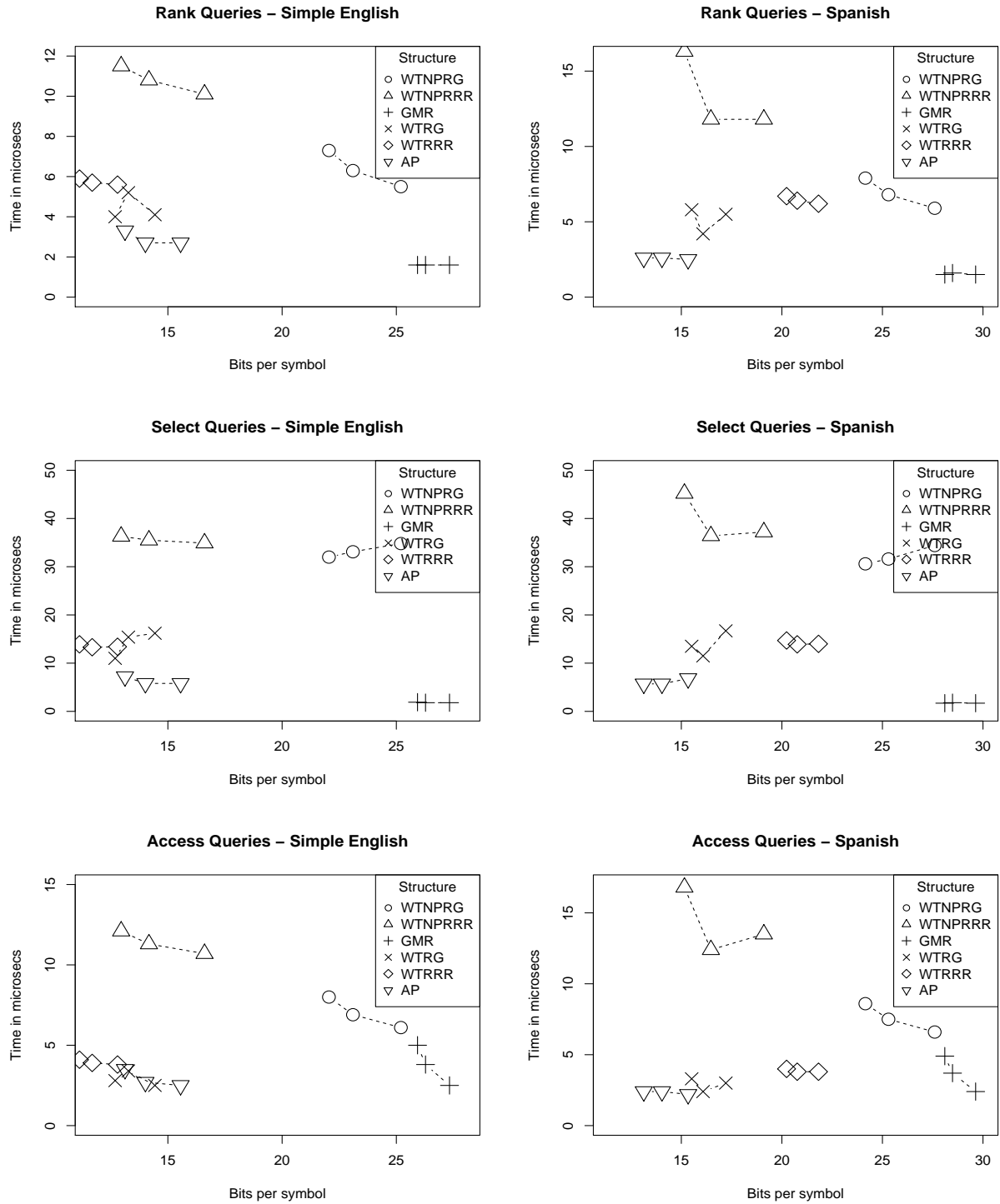
Figure 2: Time for the three operations. The x axis starts at the entropy of the sequence.
