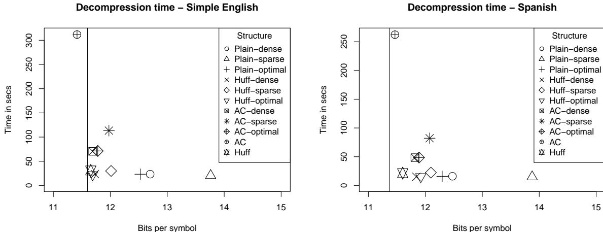
Figure 1: Space versus decompression time for basic and alphabet-partitioned schemes. The vertical line marks the zero-order entropy of the sequences. AC can slightly break the entropy barrier on Simple English because it is adaptive.
