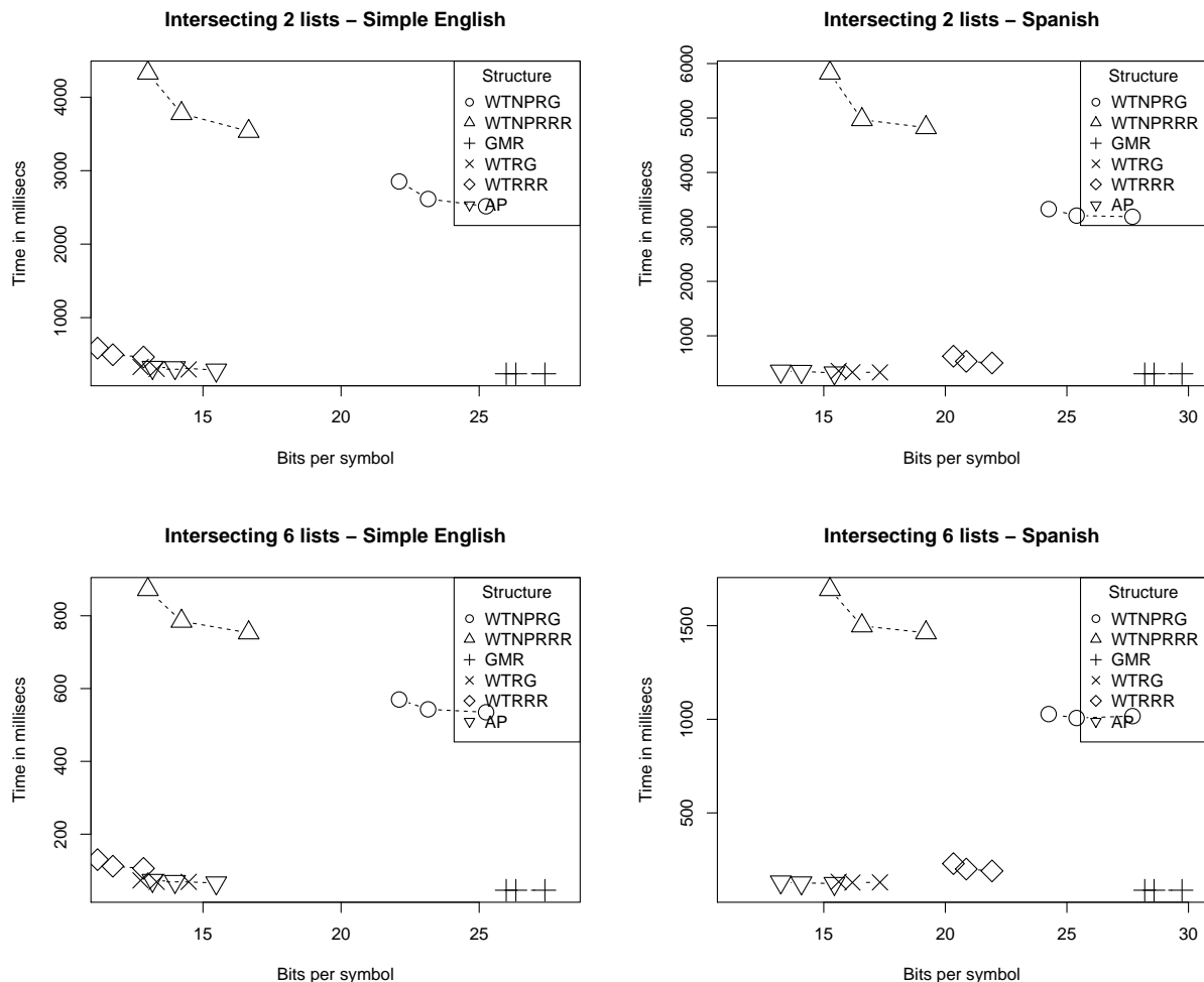
Figure 3: Results for intersection queries. The x axis starts at the entropy of the sequence.
